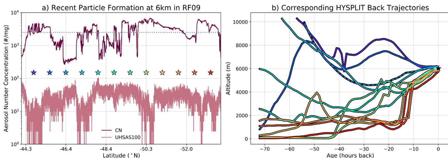
Fig. 7. (a) Time series of total CN ( D > 11 \text{ nm} ) and accumulation mode (wing mounted UHSAS, 100 < D < 1,000 \text{ nm} ) aerosol number concentrations sampled in the free tropospheric survey leg ( \sim 6 \text{ km} ) of RF09 as the G-V flew south. (b) HYSPLIT 72-h back trajectories of air masses initiated in 10-min intervals [starred locations in (a) with color-coded matched time in (b)] along the G-V flight path. Trajectories dominated by RPF events are identified by where maximum CN over the corresponding 10 min exceeds 2,500 \text{ mg}^{-1} [dotted line in (a)]. In this case, only one trajectory does not satisfy the criteria for RPF events [dashed line in (b)]. The majority of trajectory ascents exhibit synoptic uplift ( 3\text{--}6 \text{ cm s}^{-1} ) within 20–30 h of SOCRATES sampling (star) and are in proximity to phytoplankton emissions ( Z < 1 \text{ km} ) in the prior 72 h.
