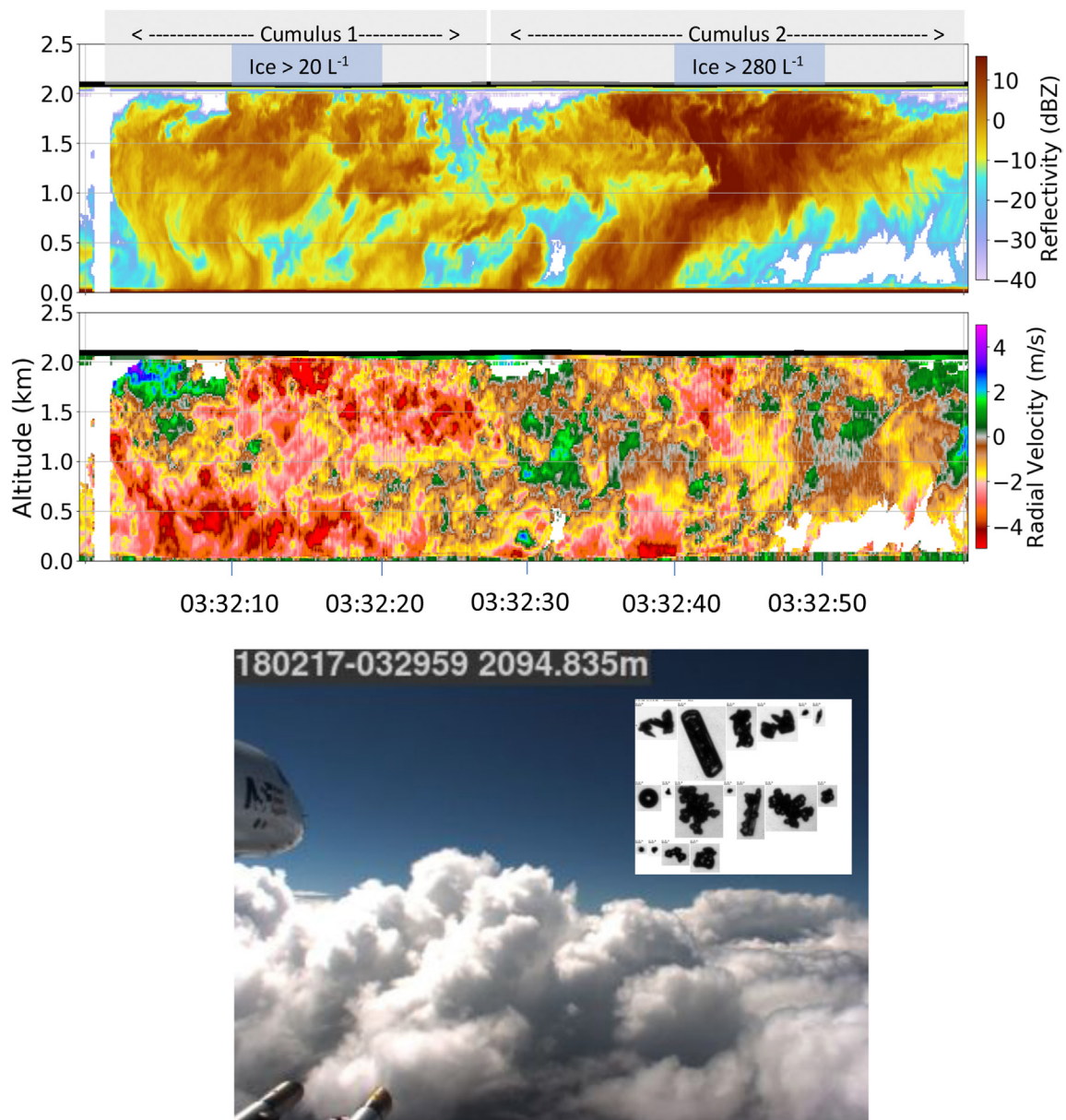
Fig. 14. Aircraft pass on 17 Feb 2018, through the tops of two closely spaced cumuli at a temperature of -9^{\circ}\text{C} , as shown by the downward-pointing airborne Doppler radar on the G-V aircraft [(top) radar reflectivity and (middle) vertical velocity; positive values denote upward motion of particles]. The black horizontal line at the top shows the aircraft location as it passed through the cloud tops. Shaded gray boxes demarcate the two clouds, with shaded blue boxes identifying 10-s regions with the highest maximum ice number concentrations (corrected for possible shattering artifacts) as labeled. (bottom) Snapshot from forward video also shows the multiple thermal structure of these cumuli as the aircraft approached. (inset) Particle images from PHIPS probe indicated rimed ice and liquid drops were present, necessary for rime splintering to be active, as well as the expected products of rime splintering, pristine, and rimed columns.
