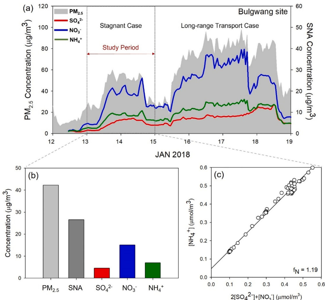
Fig. 2. (a) Temporal variations of measurements, (b) speciated mean mass concentrations of PM 2.5 , SNA, SO 4 2- , NO 3 - , and NH 4 + concentrations measured at Bulgwang site from 12 to 19 January 2018, and (c) acid aerosol neutralization parameter as given by the molar ratio of [NH 4 + ] to 2[SO 4 2- ] + [NO 3 - ].
