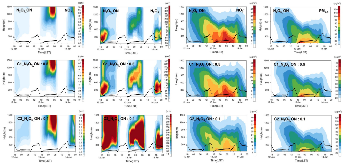
Fig. 7. Time series of vertical \text{NO}_3 , \text{N}_2\text{O}_5 , \text{NO}_3^- , and \text{PM}_{2.5} concentrations from 13 to 14 January 2018 at Bulkwang site [model: \text{N}_2\text{O}_5\text{-ON} (base case), and \text{C}_1\text{-N}_2\text{O}_5\text{-ON} (base \gamma\text{N}_2\text{O}_5 \times 0.5 , base \gamma\text{N}_2\text{O}_5 \times 0.1 )]. Black dots ( · ) represent the simulated planetary boundary layer heights.
