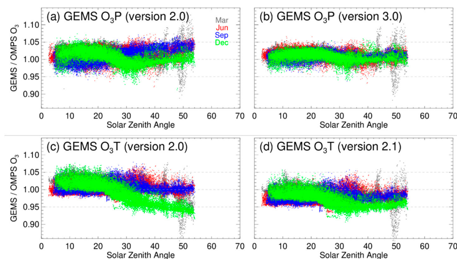
Figure 5. GEMS (04:45 UTC)-to-OMPS total ozone column ratios as a function of SZA for GEMS O 3 P ((a): version 2.0, (b): version 3.0) and O 3 T ((c): version 2.0, (d): version 2.1). Colors represent observations from 15 March, 15 June, 15 September, and 15 December 2021. Among the GEMS reference times, 04:45 UTC is close to the OMPS overpass time over East Asia.
